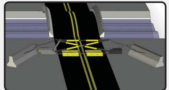
Suggested concepts for passive barrier system connections
